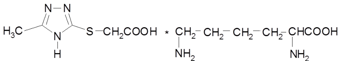
Fig. 1. L-lysine 3-methyl-1.2.4-triazole-5-thioacetate
