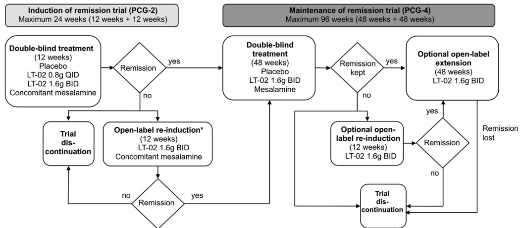
Supplementary Figure 1. Study design. *Patients who completed the double-blind treatment period as scheduled but did not achieve remission or discontinued the trial after at least 8 weeks of treatment because of lack of efficacy and with no improvement in mDAI (decrease by \leq 1 ) had the option to continue in an open-label sub-trial.
