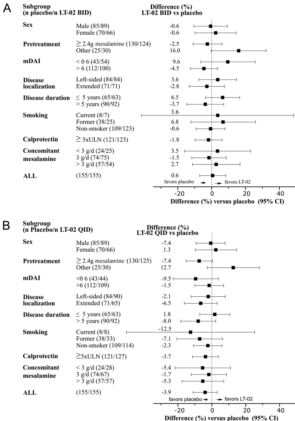
Supplementary Figure 3. PCG-2: Differences in proportions of patients with deep remission (primary end point) at week 12 (LOCF) between the BID regimen and placebo (A) or the QID regimen versus placebo (B) stratified by baseline characteristics. Deep remission was defined as mDAI score ≤ 1 with 0 points for rectal bleeding and stool frequency, and ≥ 1-point reduction from baseline in the mucosal appearance score, at week 12 (LOCF). P values (one-sided) were based on \chi^2 test for comparison against placebo; 95% CIs were based on normal approximation. LOCF, last observation carried forward; ULN, upper limit of normal.
